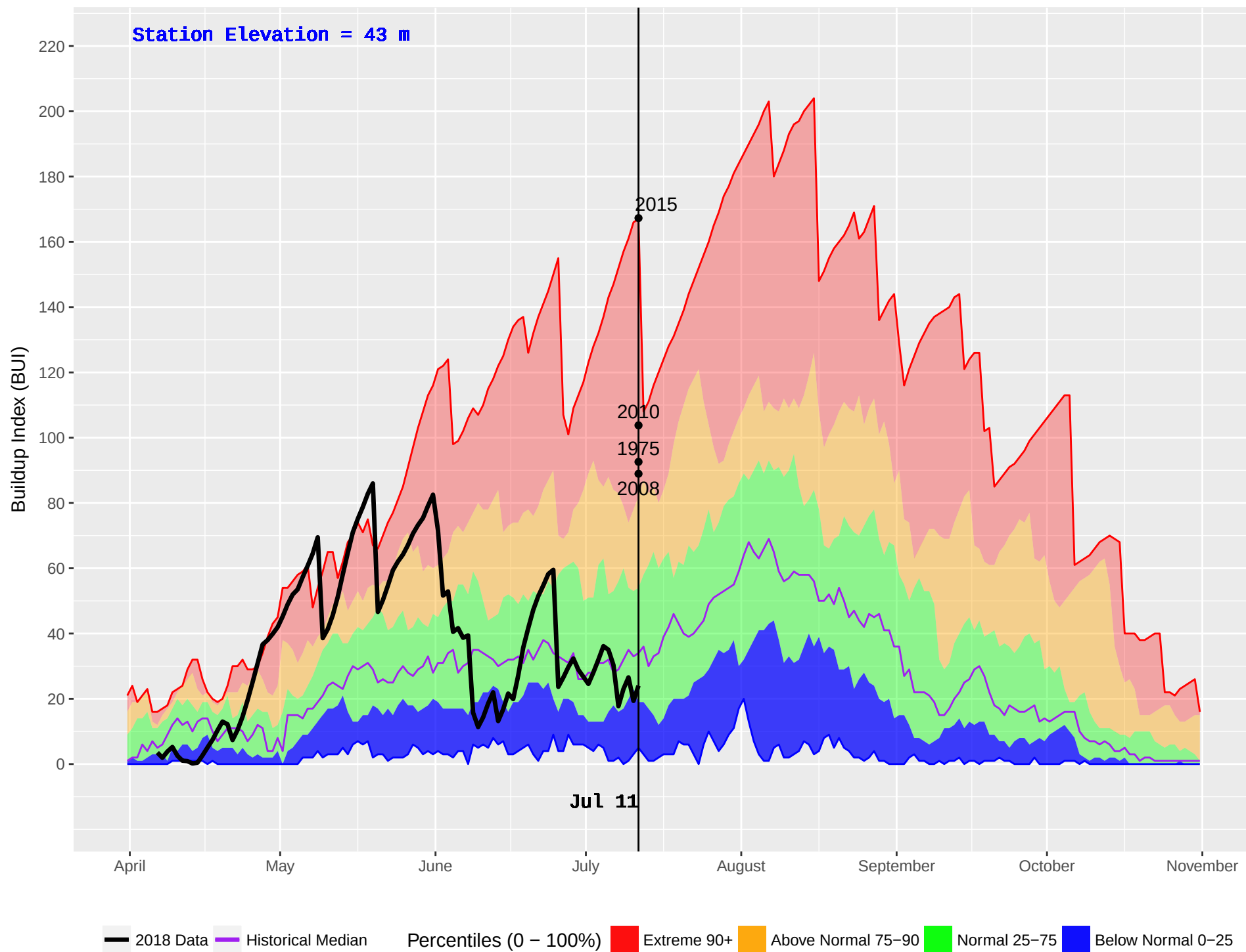
TOBA CAMP (75) : Historical (1970–2016) and Current (2018) Noon Buildup Index (BUI)
