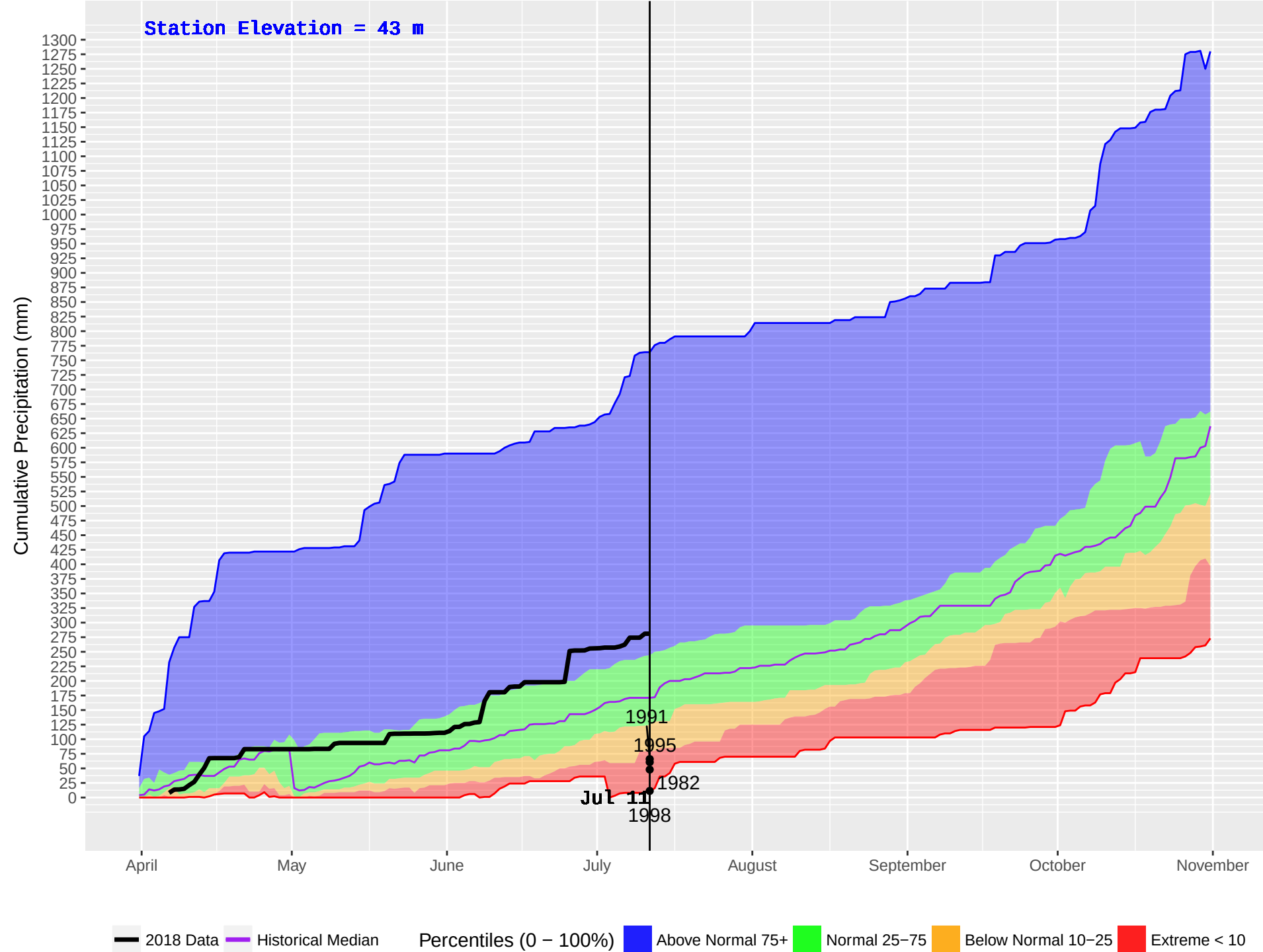
TOBA CAMP (75) : Historical (1970–2016) and Current (2018) Noon Cumulative Precipitation
