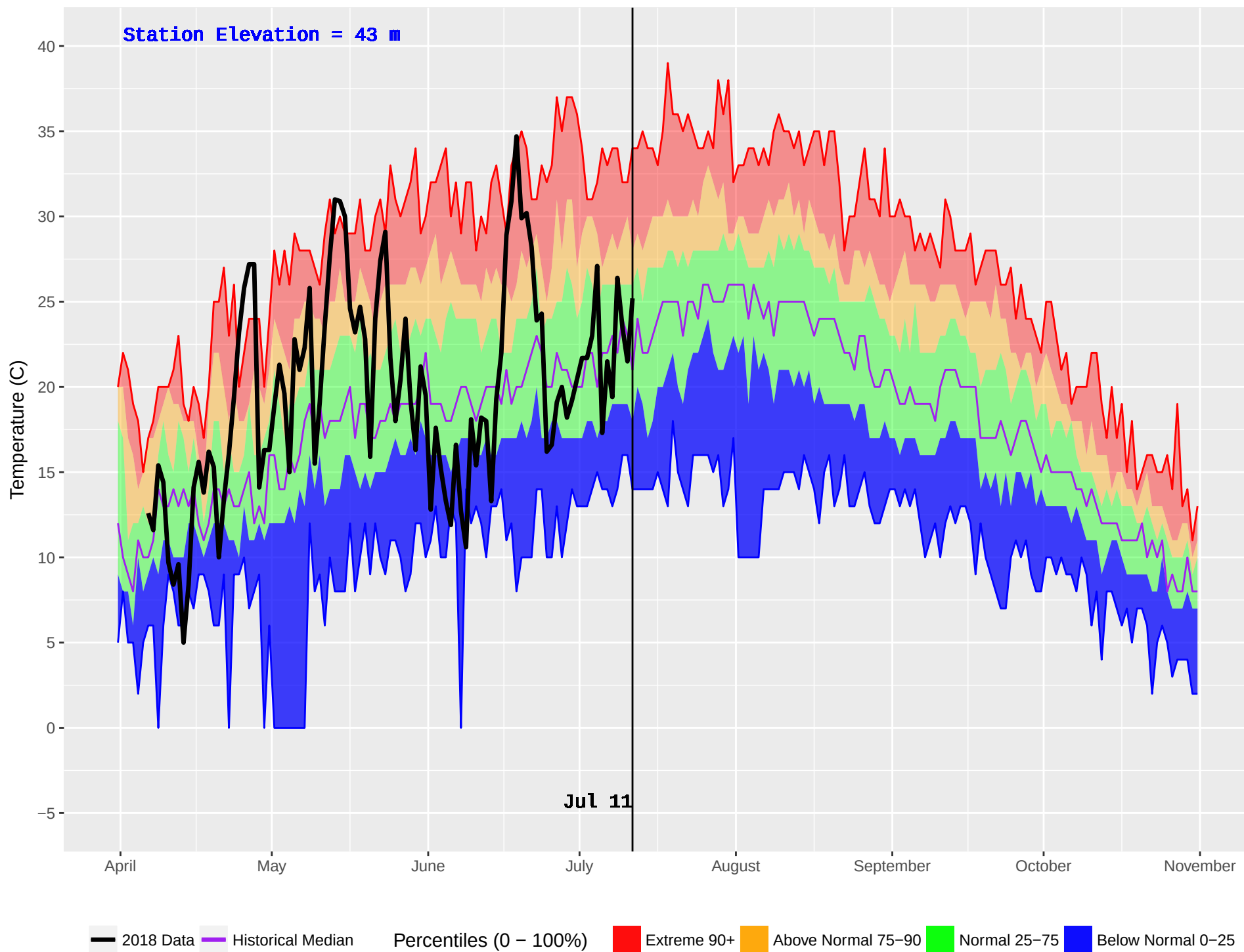
TOBA CAMP (75) : Historical (1970–2016) and Current (2018) Noon Temperature
