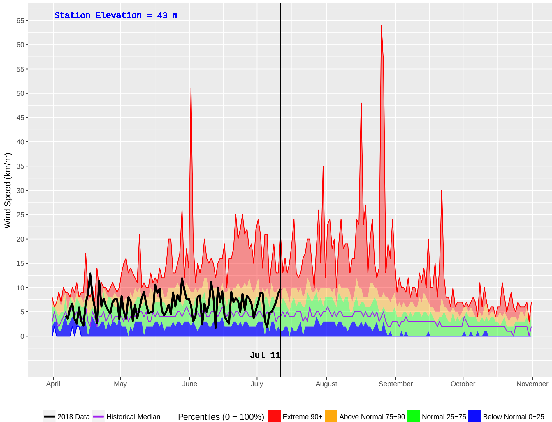
TOBA CAMP (75) : Historical (1970–2016) and Current (2018) Noon Wind Speed
