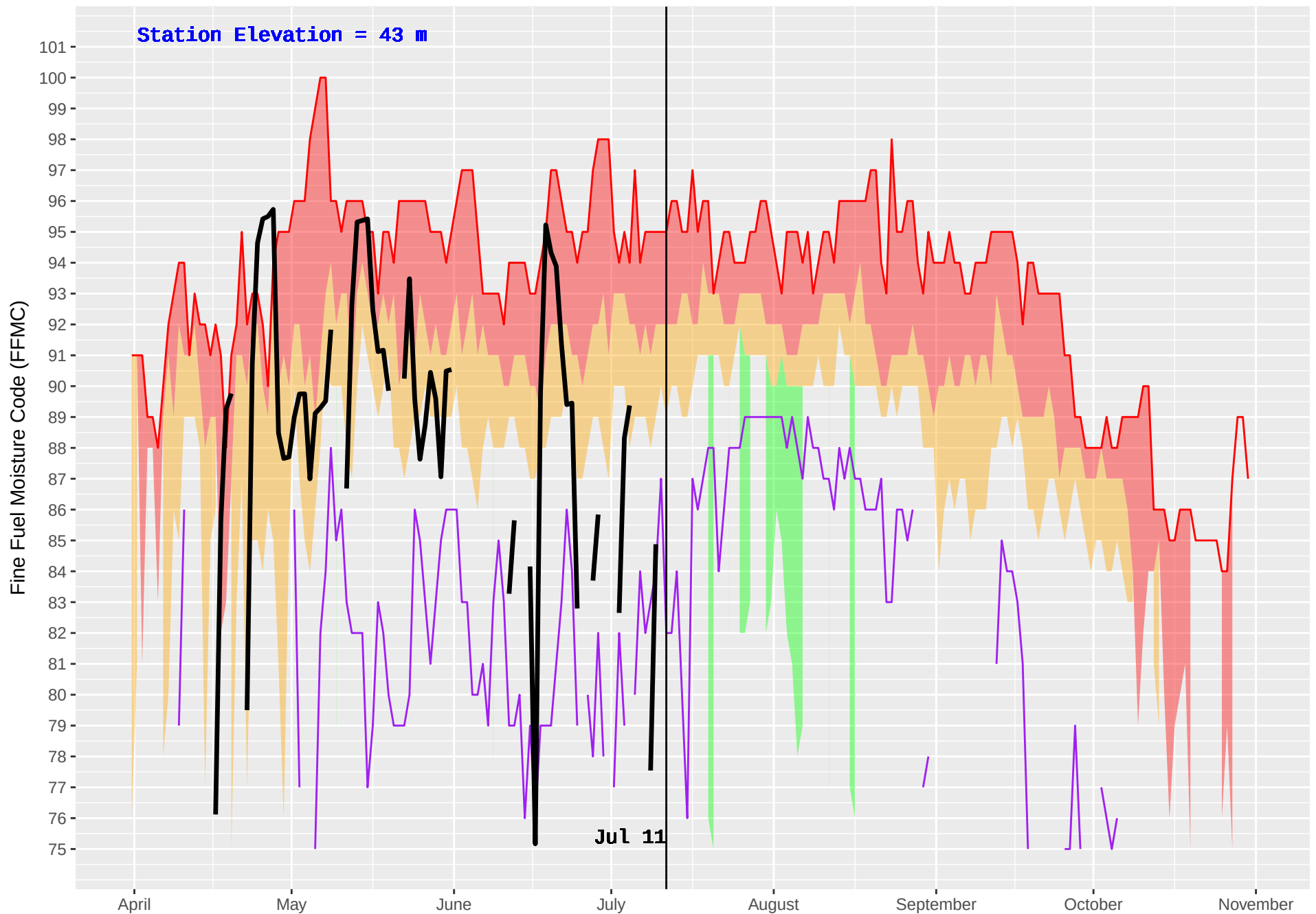
TOBA CAMP (75) : Historical (1970–2016) and Current (2018) Noon Fine Fuel Moisture Code (FFMC)
