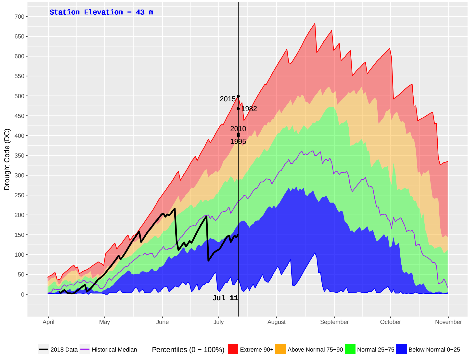
TOBA CAMP (75) : Historical (1970–2016) and Current (2018) Noon Drought Code (DC)
