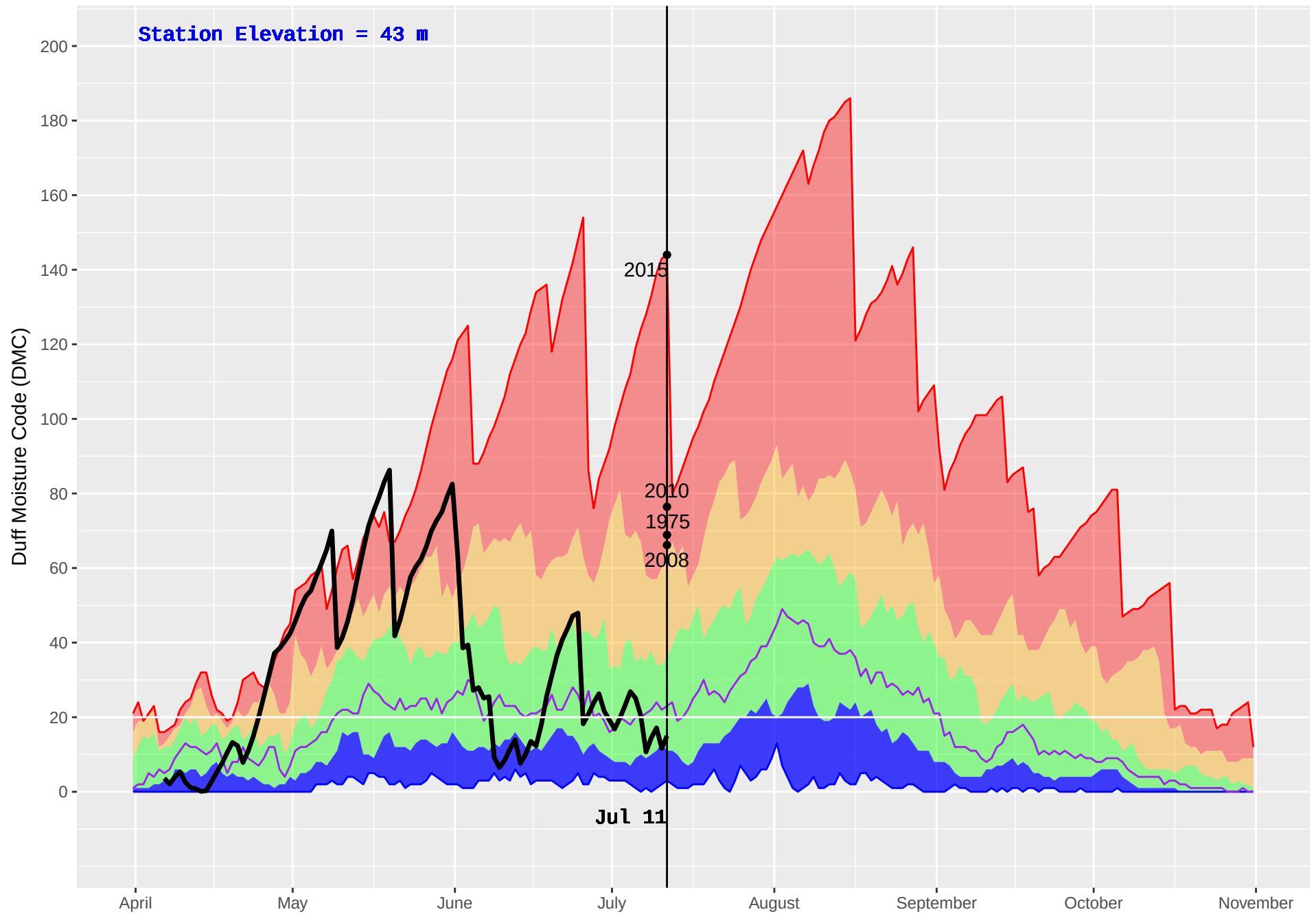
TOBA CAMP (75) : Historical (1970–2016) and Current (2018) Noon Duff Moisture Code (DMC)
