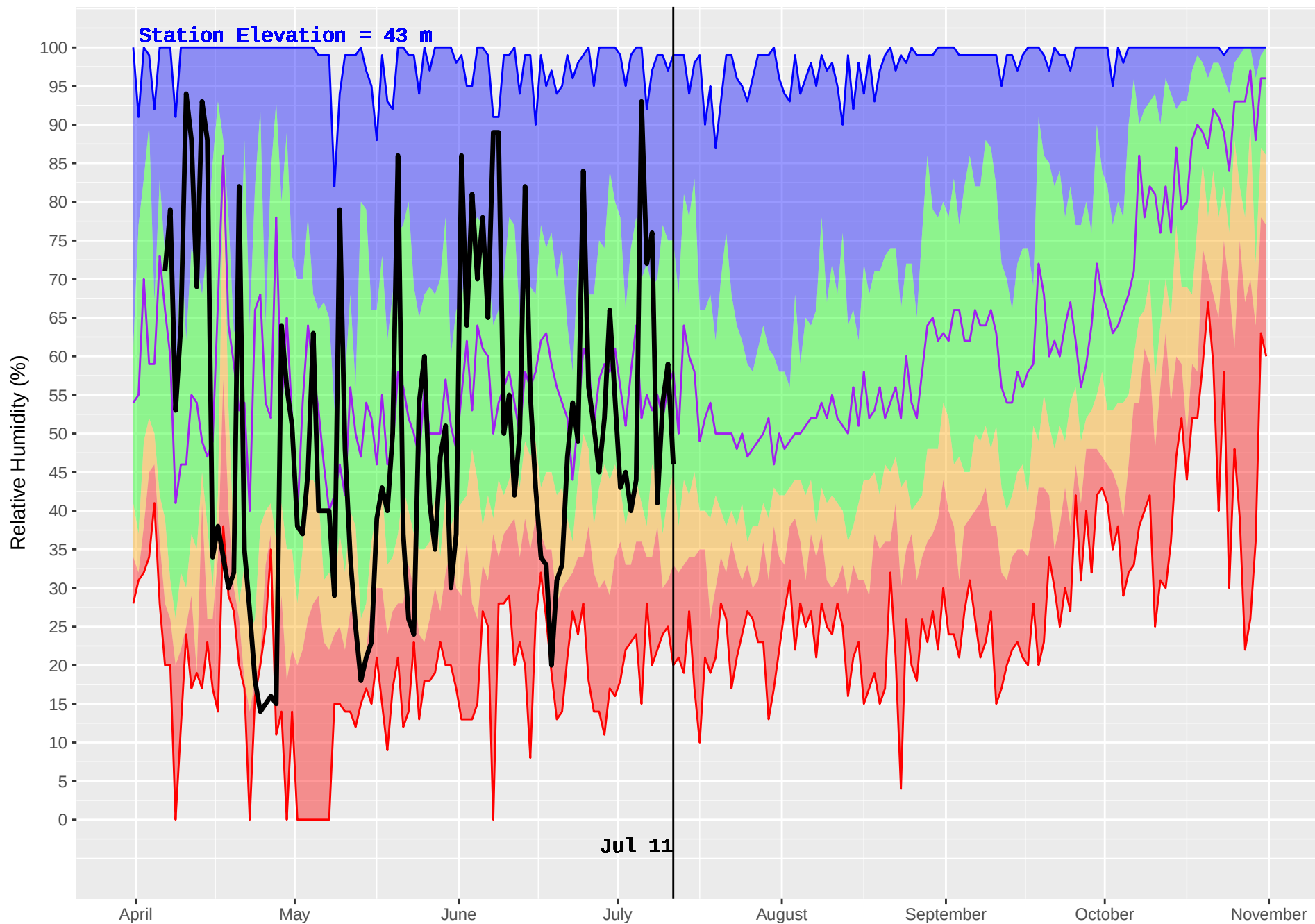
TOBA CAMP (75) : Historical (1970–2016) and Current (2018) Noon Relative Humidity
